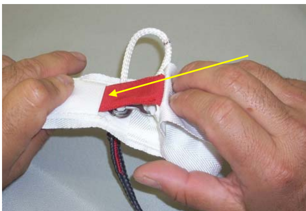
Tuck the stiffened T-III Tab into the tuck channel on top of the Long Pin Channel.
