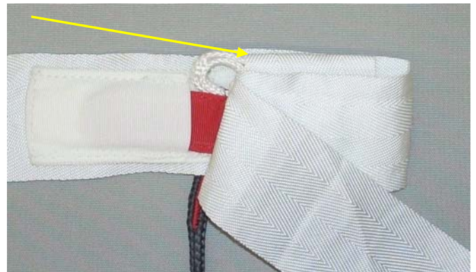
Stow the Spectra Line Loop into the polyester sleeve opposite the long pin channel.
